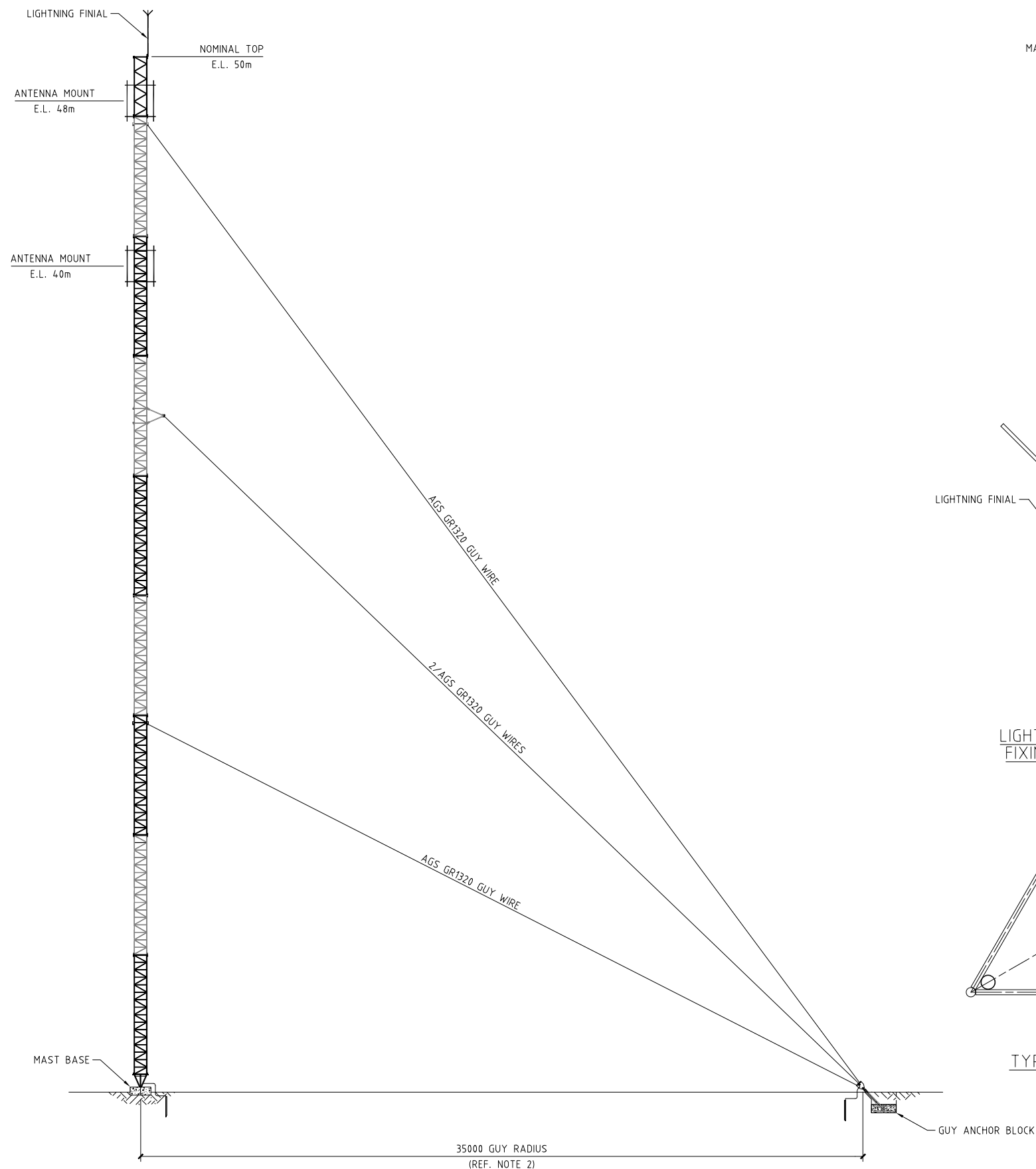
MAST ELEVATION
