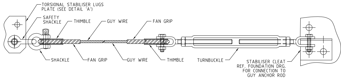
TYPICAL TORSIONAL STABILISER GUY ASSEMBLY
