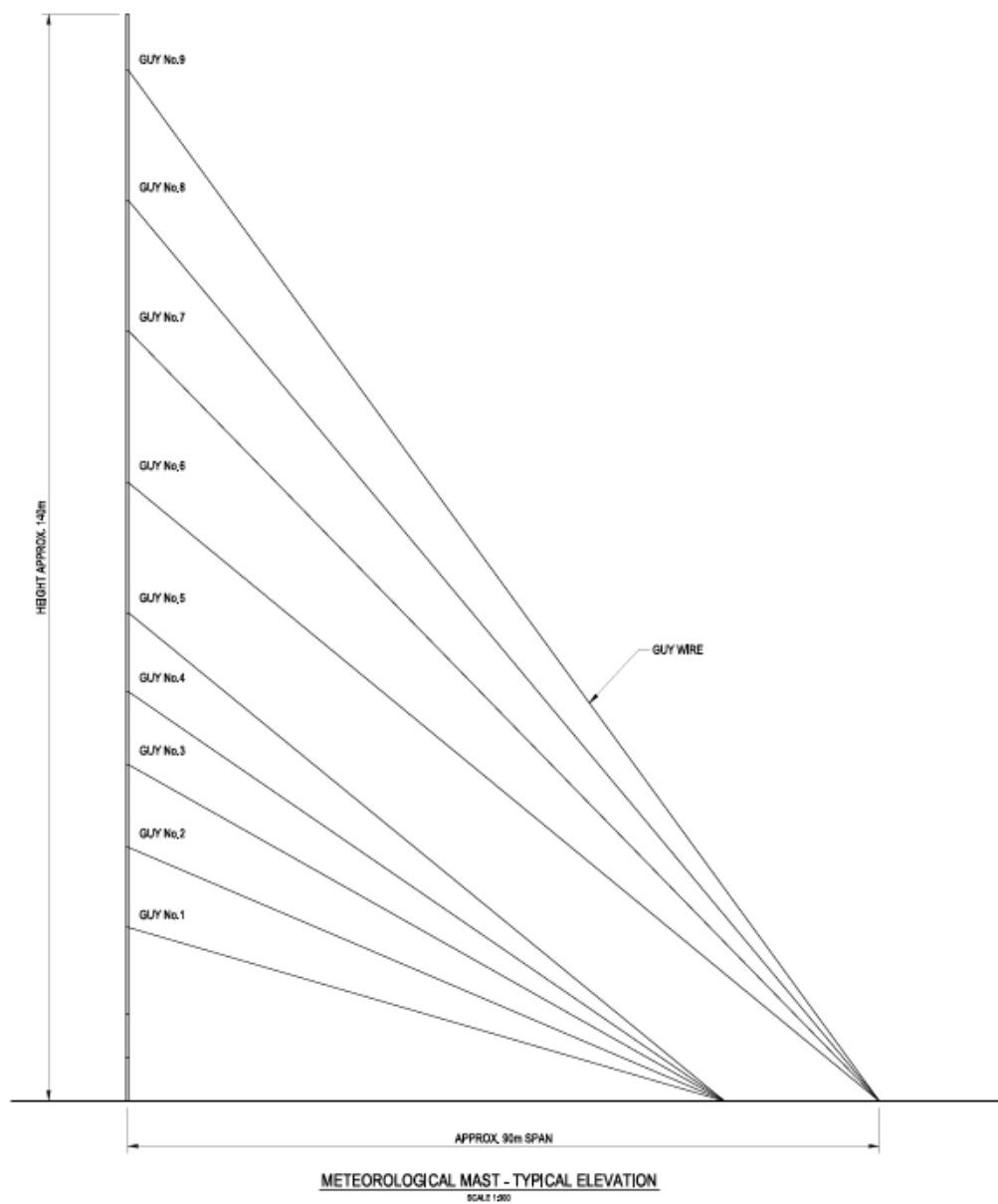
Figure 1 – Met Mast Elevation
